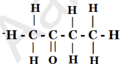
Ethanoic Acid
