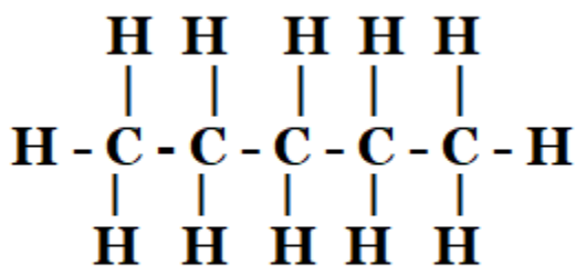
n-pentane
