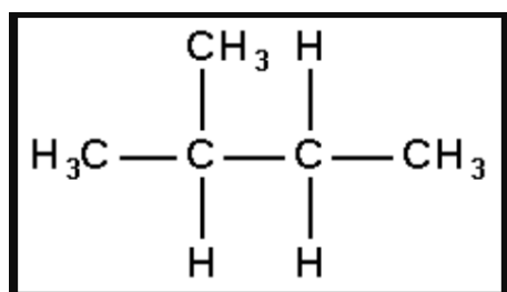
2-methylbutane
