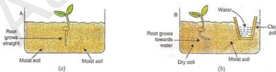
Experiment to show the response of a plant to water (hydrotropism).
