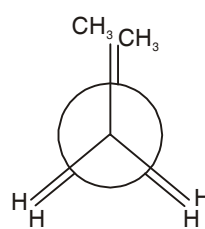
Eclipsed-conformer
