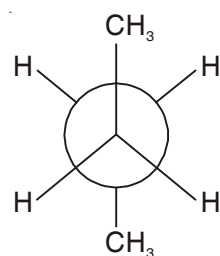
Anti-conformer
